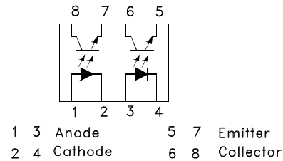
Internal connection diagram
